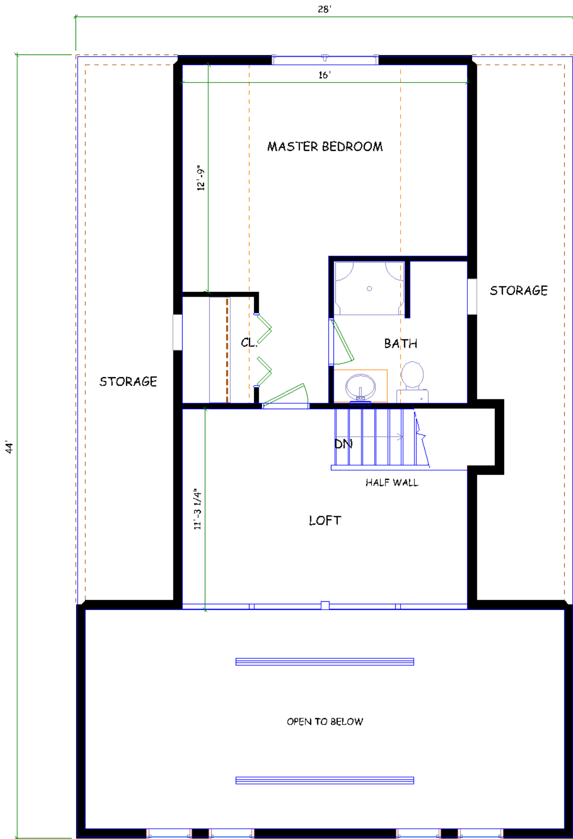
THE WYOMING 2nd FLOOR SQ. FT. = 508 sf
