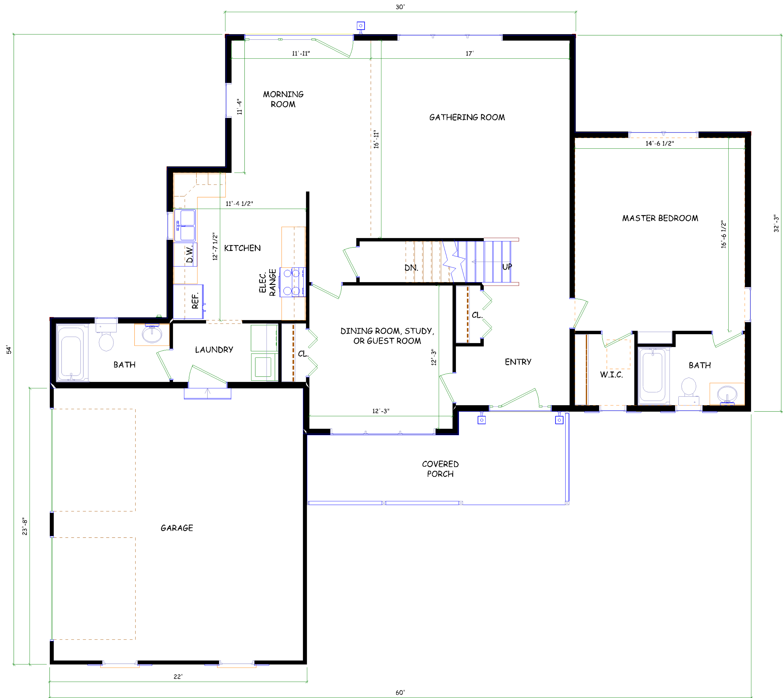
THE SULLIVAN 1st FLOOR PLAN SQ. FT. = 1,508 sf
