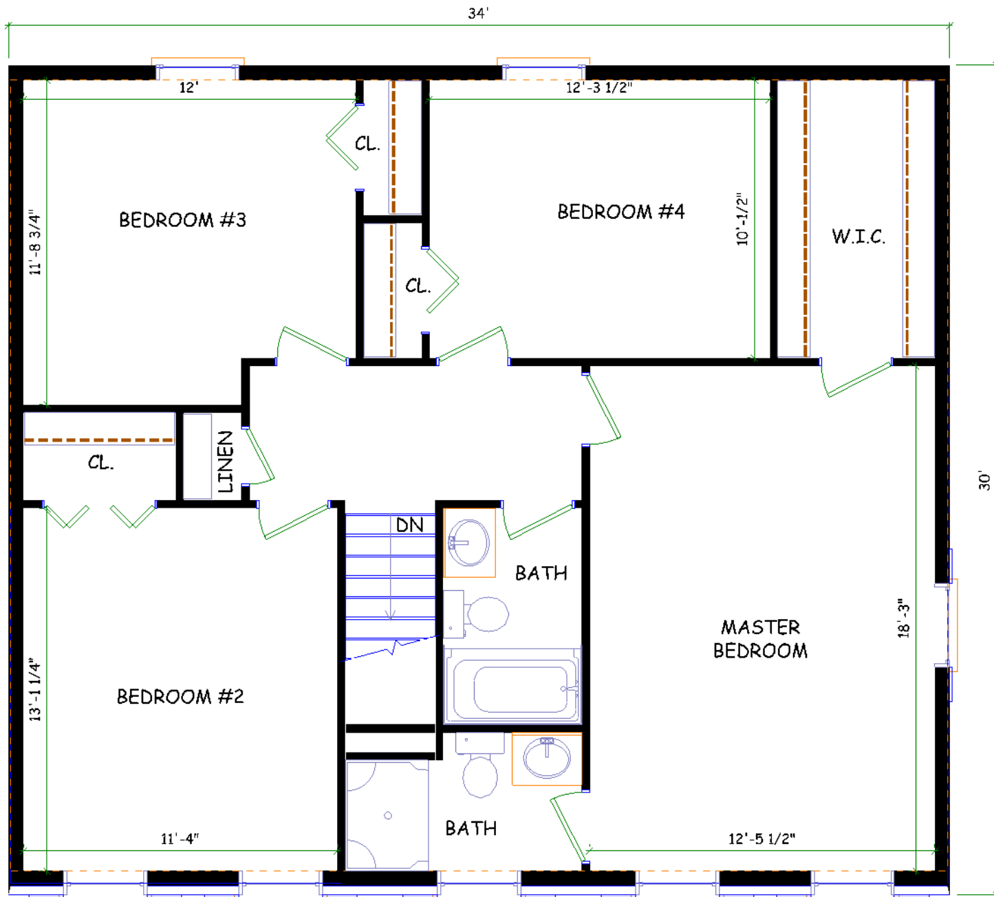
THE LANCASTER 2nd FLOOR PLAN SQ. FT. = 1,009 sf
